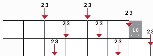
FIG. A: ABOVE EYE LEVEL, USE #23 GAUGE NAILS AT A DOWNWARD ANGLE.
