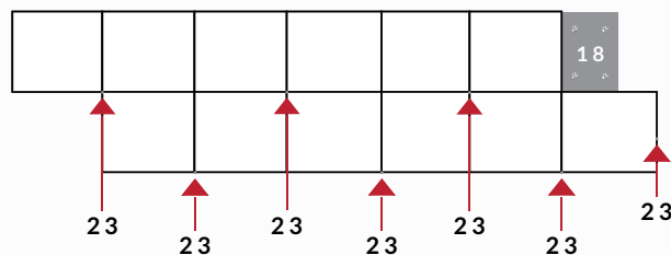
FIG. C: BELOW EYE LEVEL, USE #23 GAUGE NAILS, NAILING AT AN UPWARD ANGLE TO AVOID VISIBLE NAILS.
